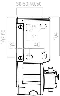
Vista frontal
